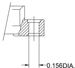
VARIATION 04 .156 +.002 -.000 DIA. MOUNTING HOLE
