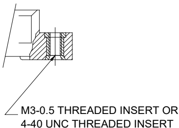
VARIATIONS 07 AND 08 THREADED INSERT
