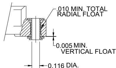
VARIATION 03 .116 +.003 -.000 I.D. FLOATING EYELET
