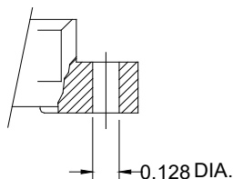
VARIATION 02 .128±.003 DIA. MOUNTING HOLE
