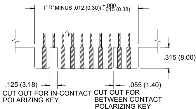
RECOMMENDED DAUGHTER BOARD
