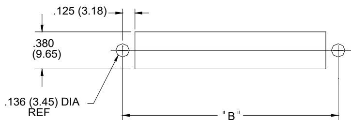
CONNECTOR MOUNTING PATTERN PANEL MOUNT CUT OUT
