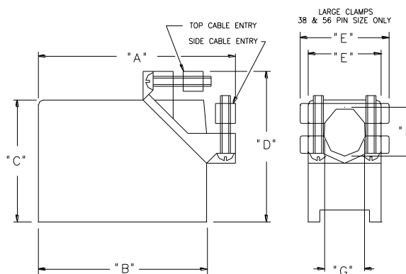
PLASTIC COVERS
