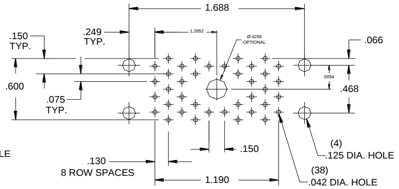
38 PINS
