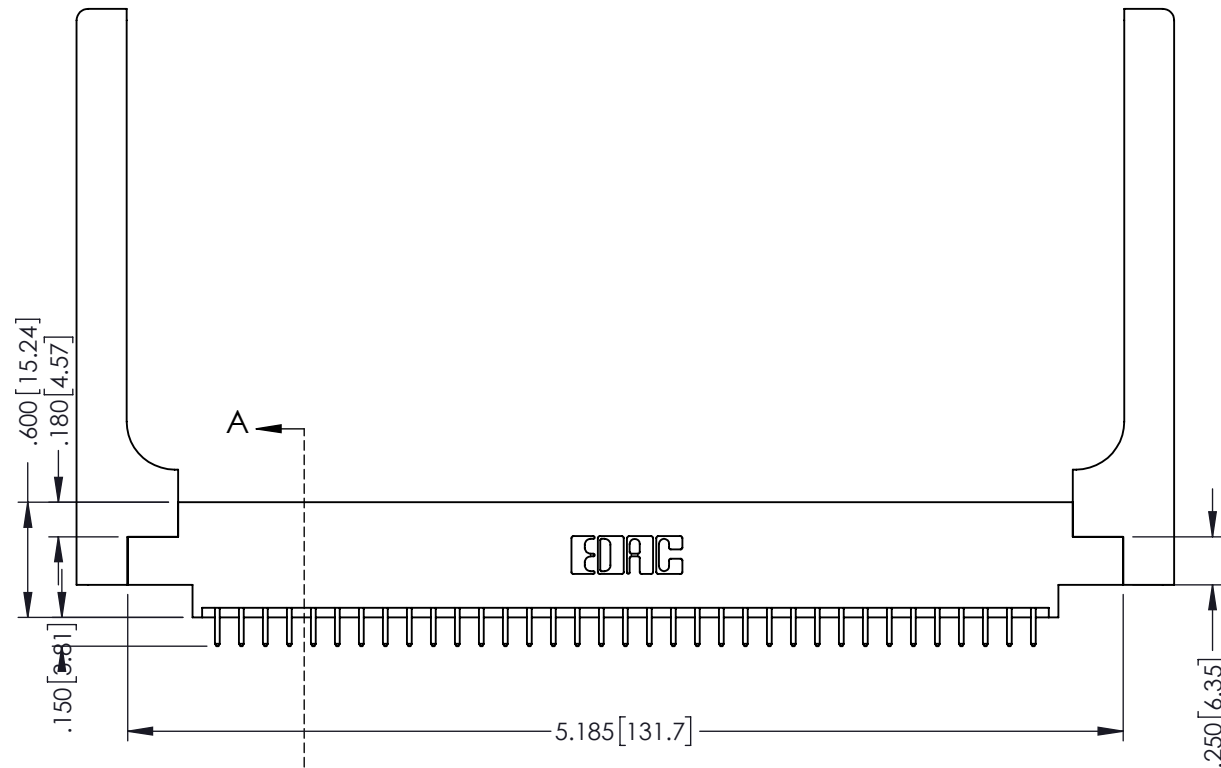
346/396 SERIES CARD EDGE CONNECTOR PART NUMBER: 396-070-521-858
