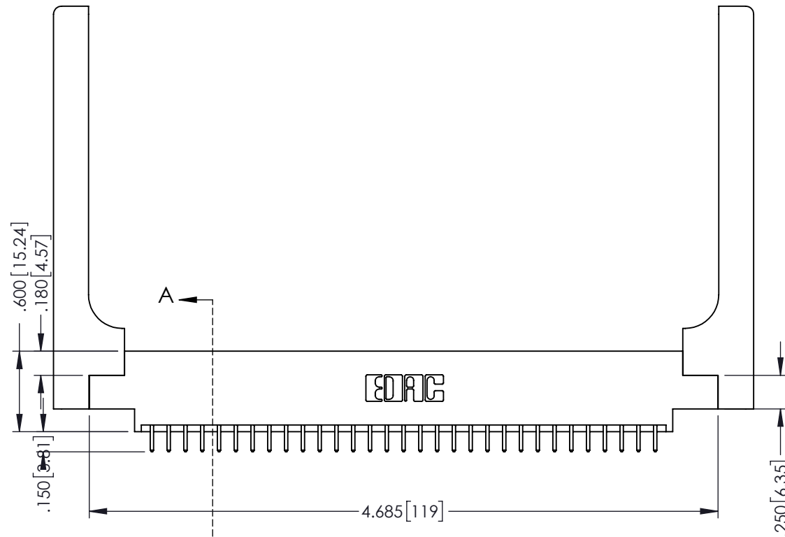
346/396 SERIES CARD EDGE CONNECTOR PART NUMBER: 396-062-521-858
