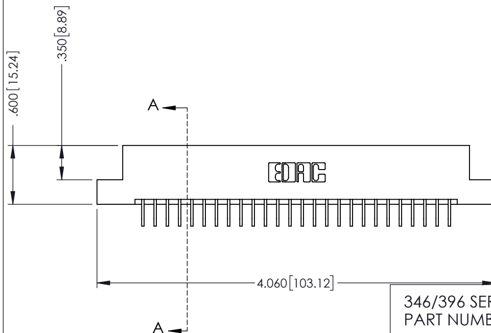
• INSULATOR MATERIAL: THERMOPLASTIC POLYESTER, UL 94V-0 • CONTACT MATERIAL: COPPER, NICKEL, TIN ALLOY CA-725 • CONTACT PLATING: GOLD ON THE MATING AREA, TIN-LEAD ON THE CONTACT TAILS, NICKEL UNDERPLATE
