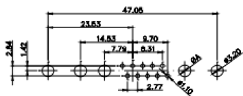
13W3 Male
