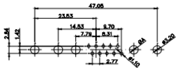
13W3 Male
