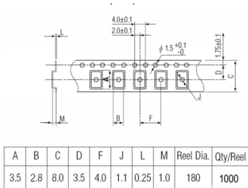
Figure 3) Pocket Tape Dimensions
