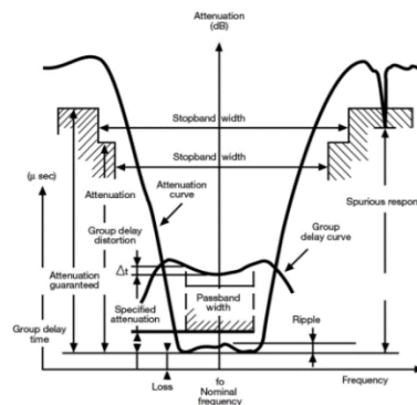
Figure 3) MCF Characteristics Curve
