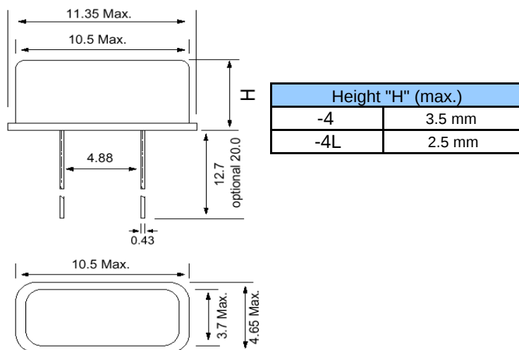
Figure 1) HC-49US-DN - Top and Side Views
