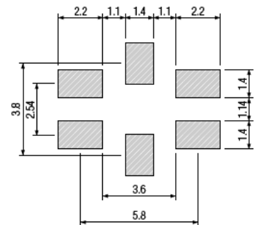
Figure 2) Land Pattern
