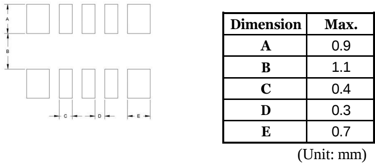
Figure 4. Recommended Soldering Pattern
