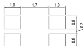
Figure 2) Suggested Land Pattern
