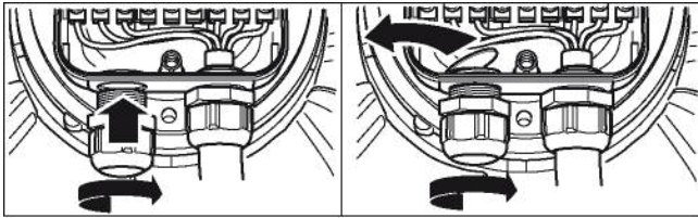
III. 3: Screwed cable gland opening
