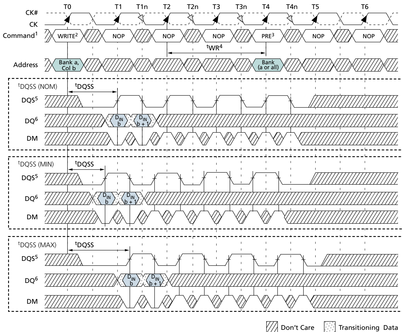
Figure 48: WRITE-to-PRECHARGE – Interrupting
