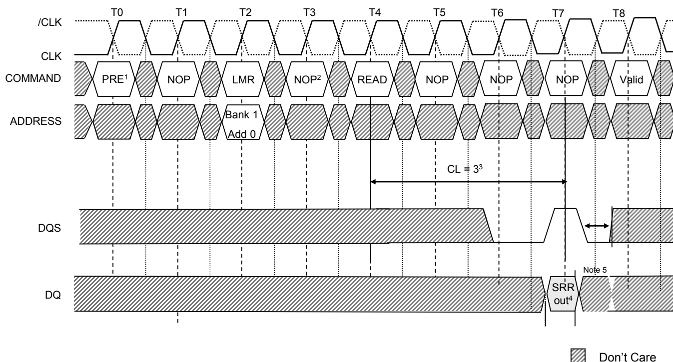
Figure 3: Status Read Register Timing
