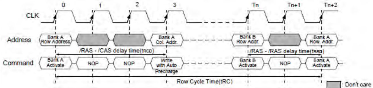
Figure 6 — Bank Activation Command Cycle
