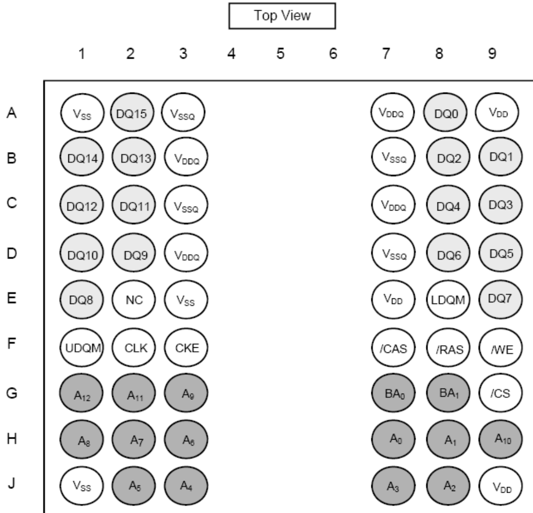
Figure 1 — PIN DESCRIPTION
