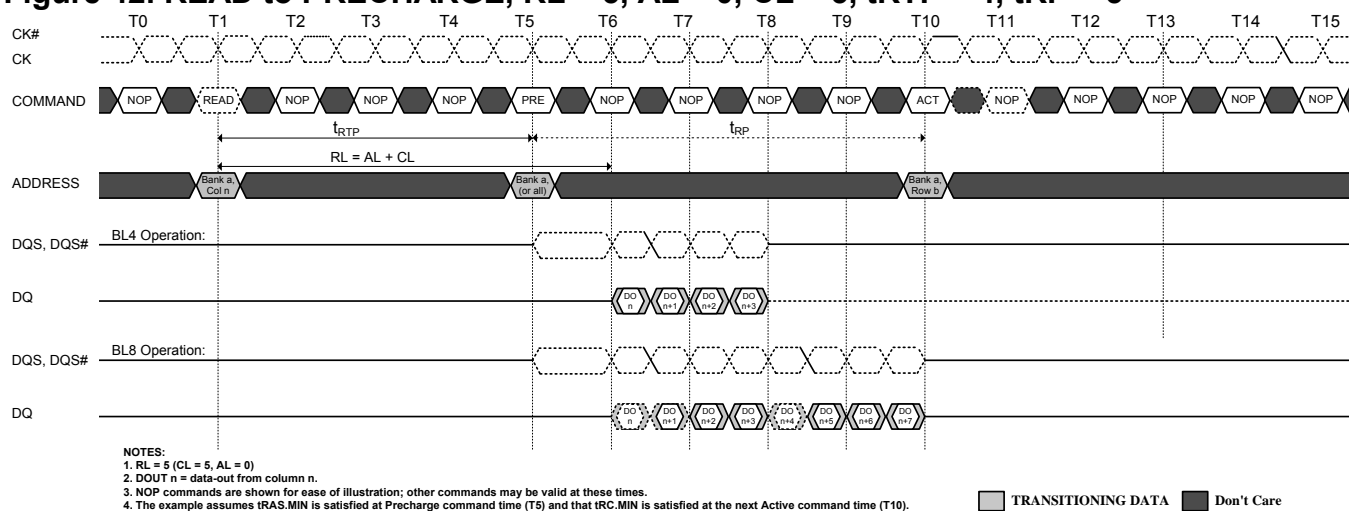
Figure 42. READ to PRECHARGE, RL = 5, AL = 0, CL = 5, tRTP = 4, tRP = 5
