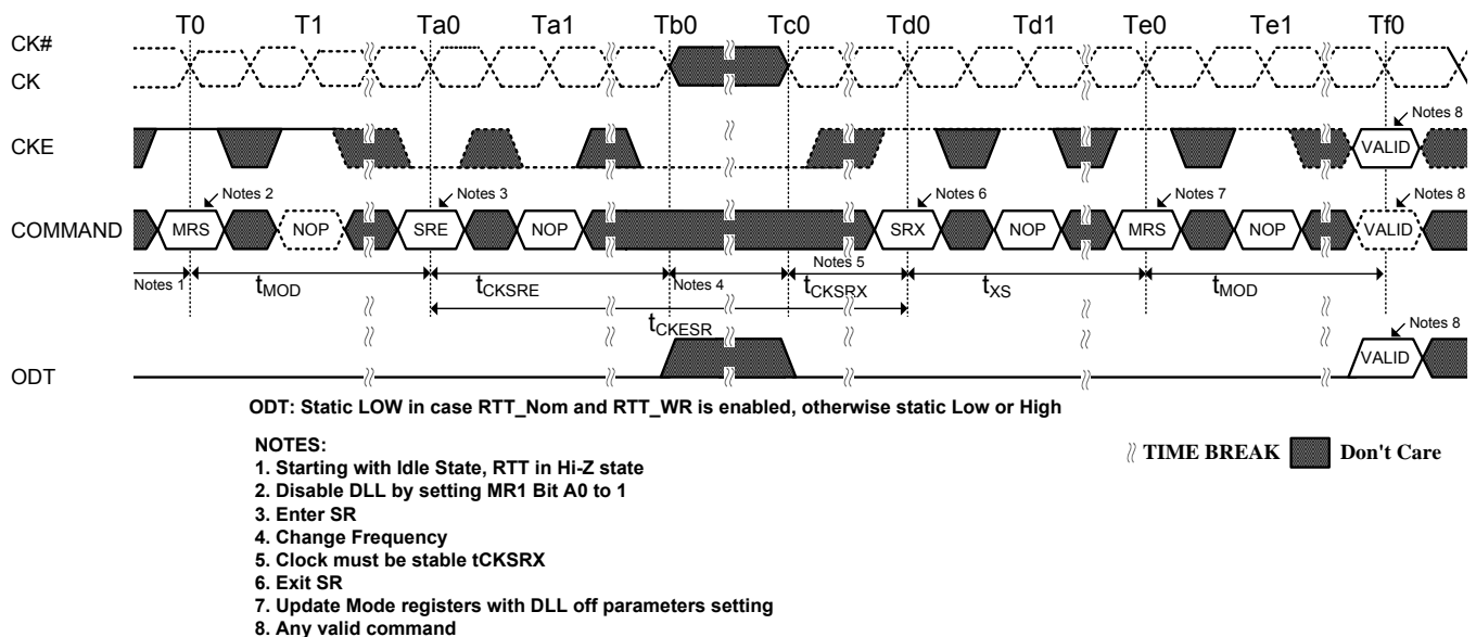
Figure 11. DLL Switch Sequence from DLL-on to DLL-off
