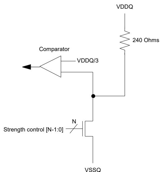
Figure 22. pull-down calibration
