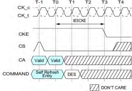
Figure 24. tESCKE Timing
