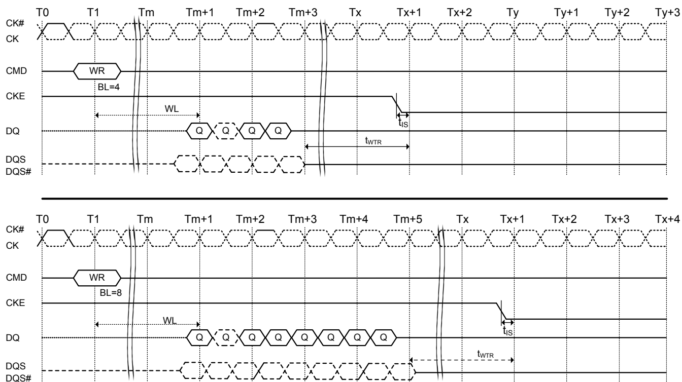
Figure 40. Write to power-down entry
