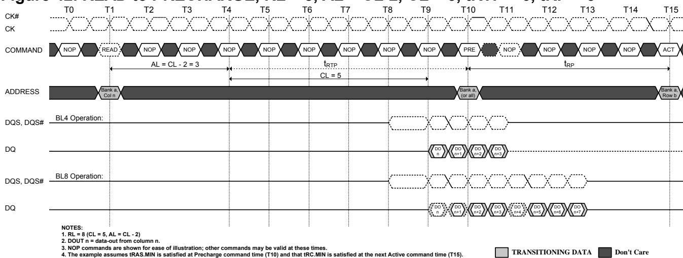
Figure 42. READ to PRECHARGE, RL = 8, AL = CL-2, CL = 5, tRTP = 6, tRP = 5
