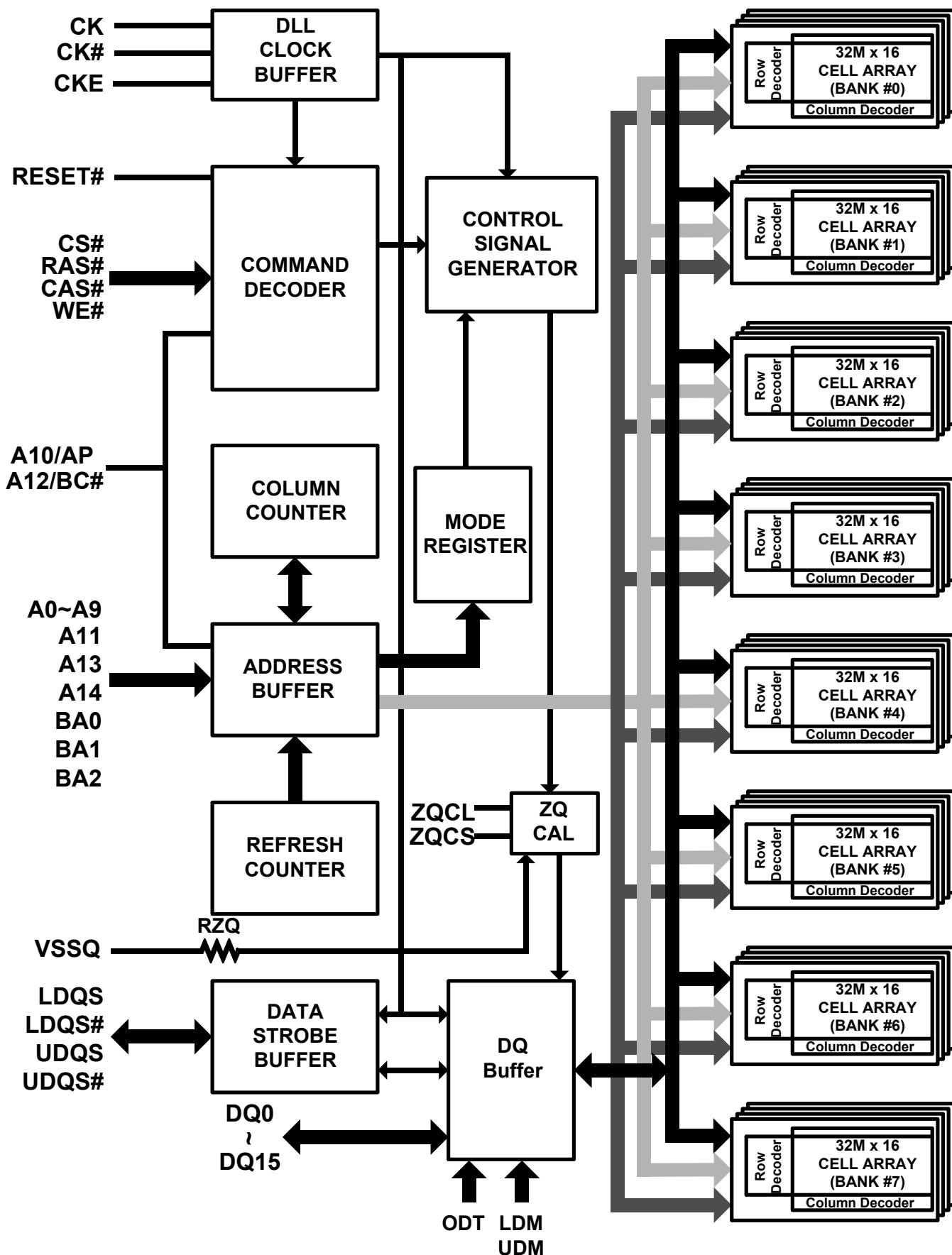
Figure 2. Block Diagram
