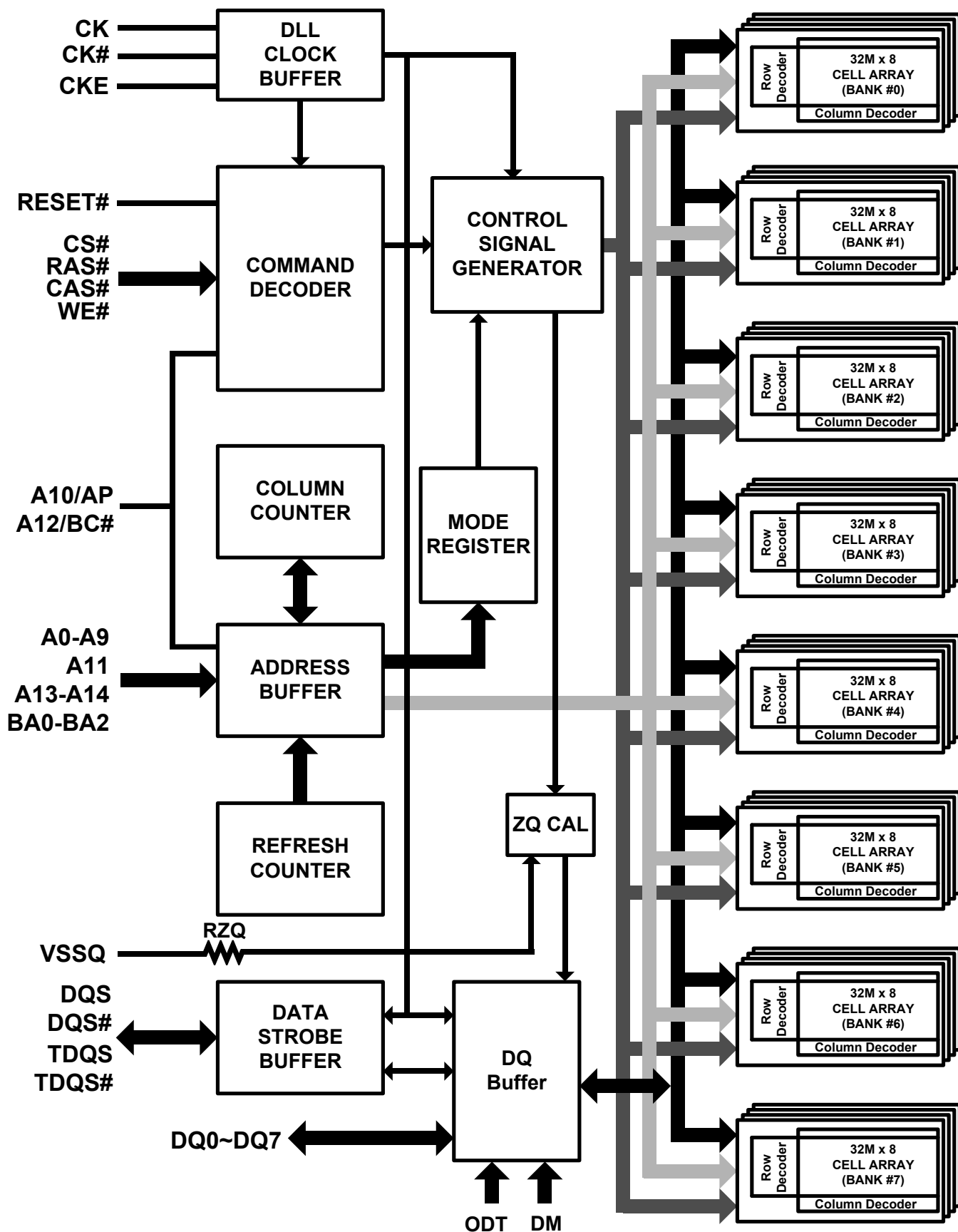
Figure 2. Block Diagram
