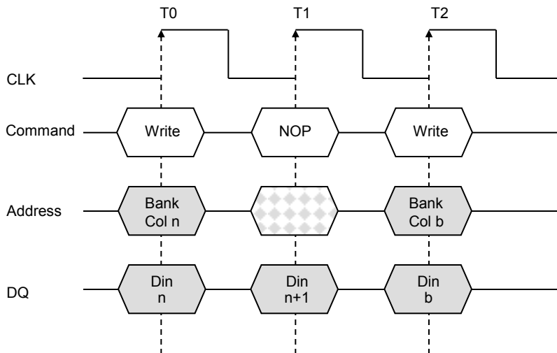
Figure 18. Write to Write - Transition from a burst of 2 to a single write
