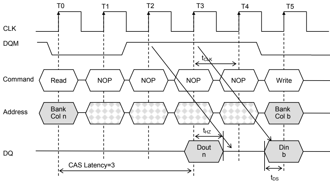
Figure 9. Read to Write with extra clock cycle
