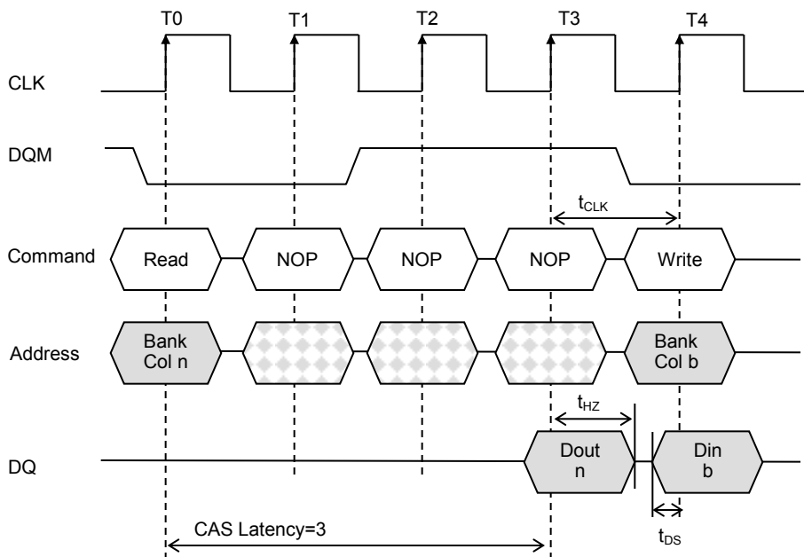
Figure 8. Read to Write
