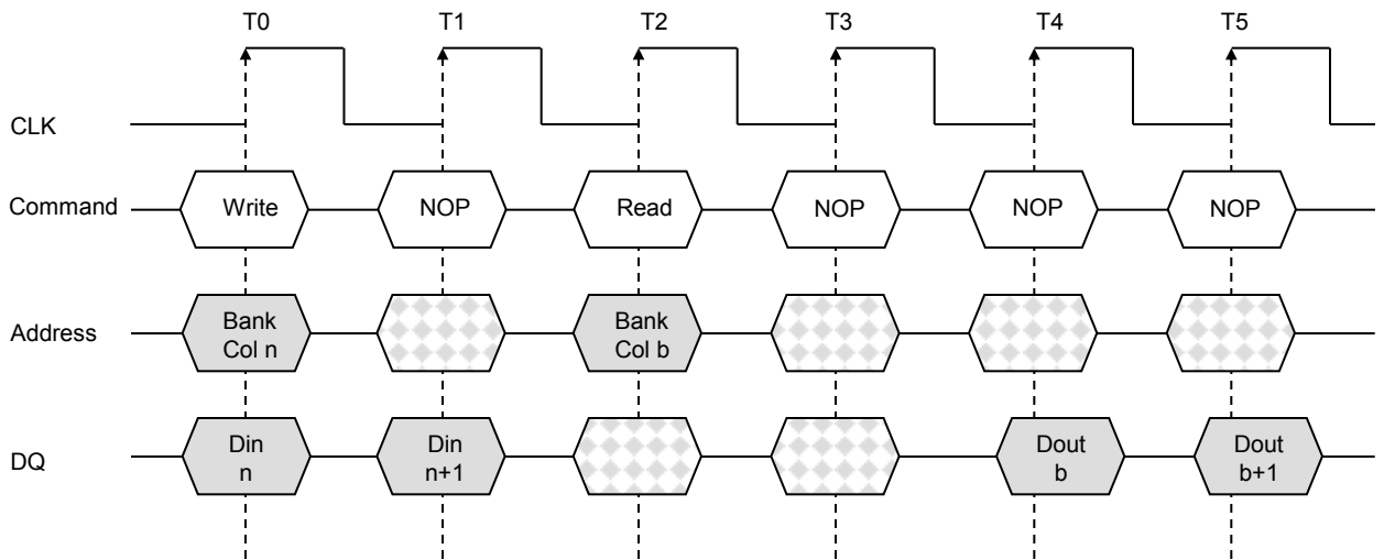
Figure 20. Write to Read Burst of 2 Write and Read(CAS Latency =2)
