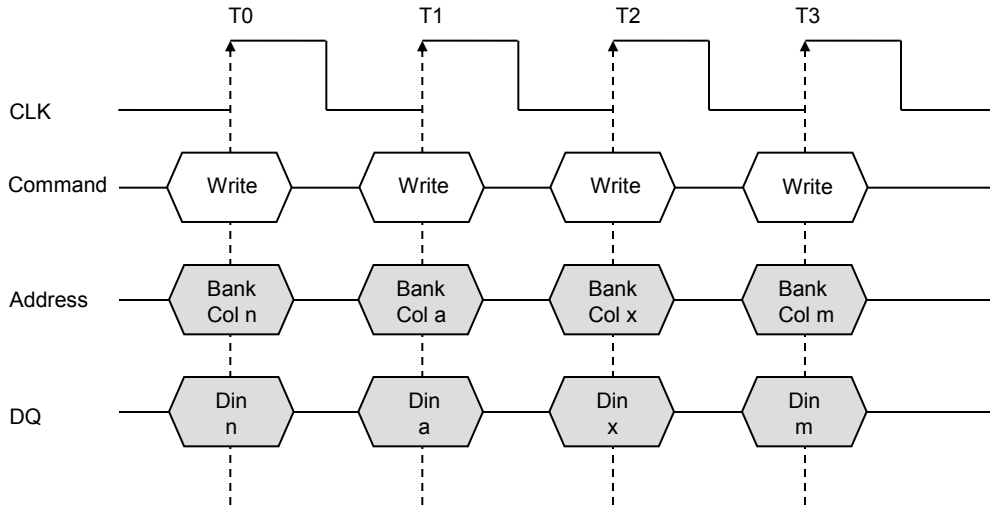
Figure 19. Random Write Cycles
