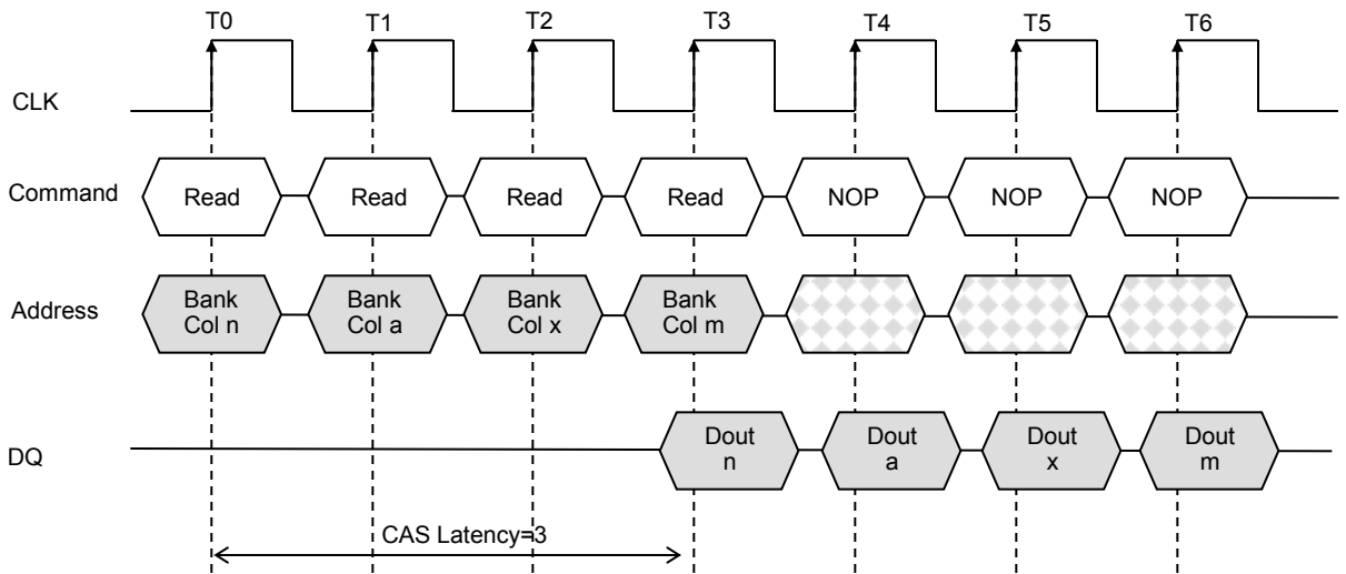
Figure 7. Random Read Accesses for CAS Latency =2,3
