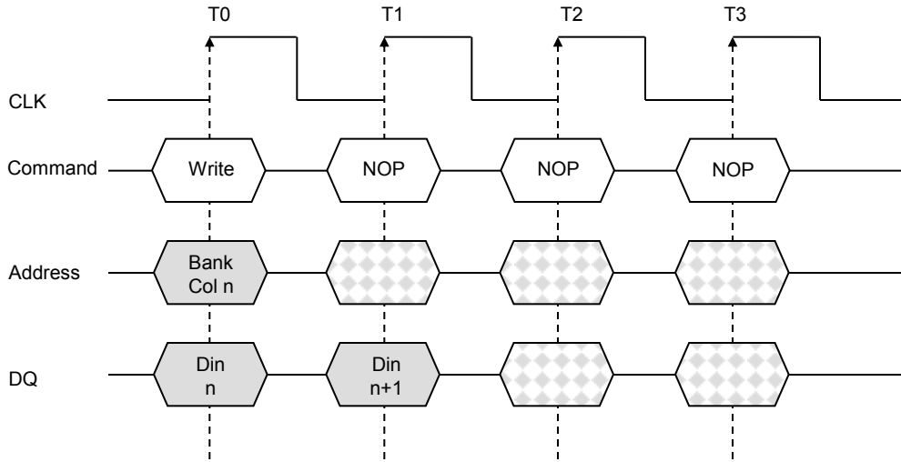
Figure 17. Write Burst - Burst length of 2
