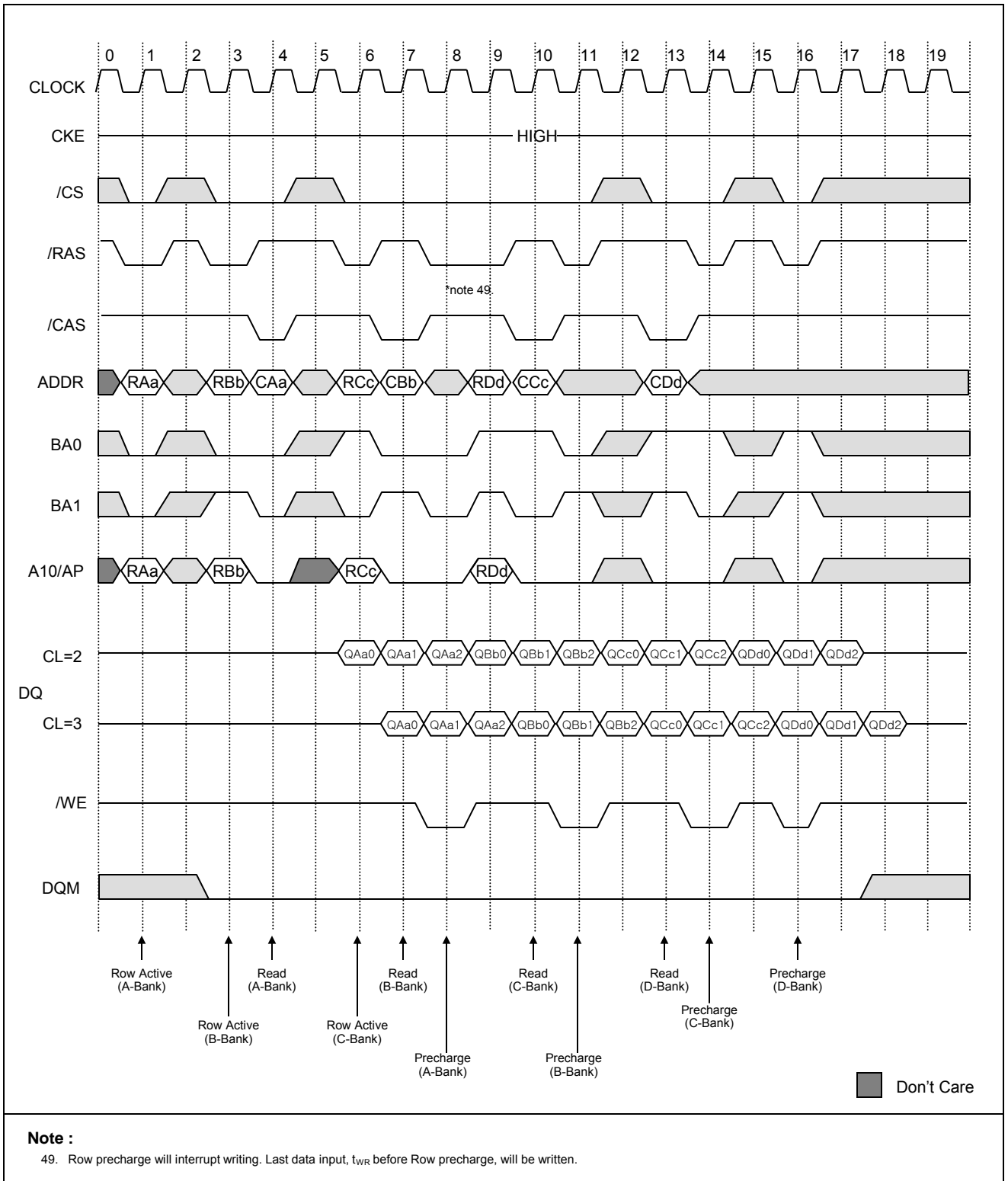
Figure 15. Page Read Cycle at Same Bank @ Burst Length=4
