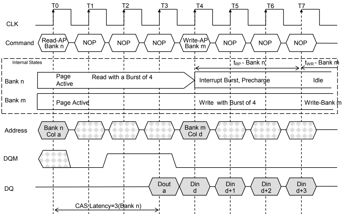
Figure 28. Read With Auto Precharge Interrupted by a Write(Read CAS Latency =3)
