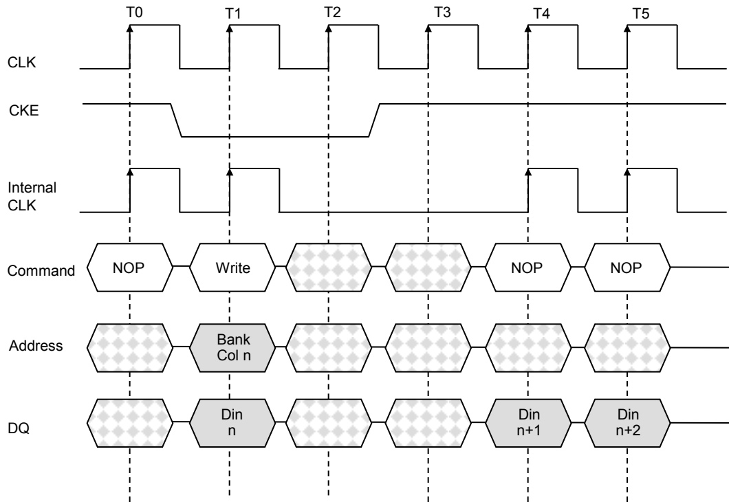
Figure 25. Clock Suspend During Write Burst
