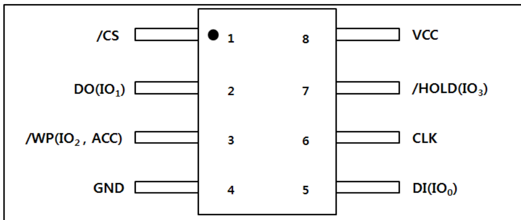
Figure 1a. Pin Assignments, 8-pin SOP 208-mil
