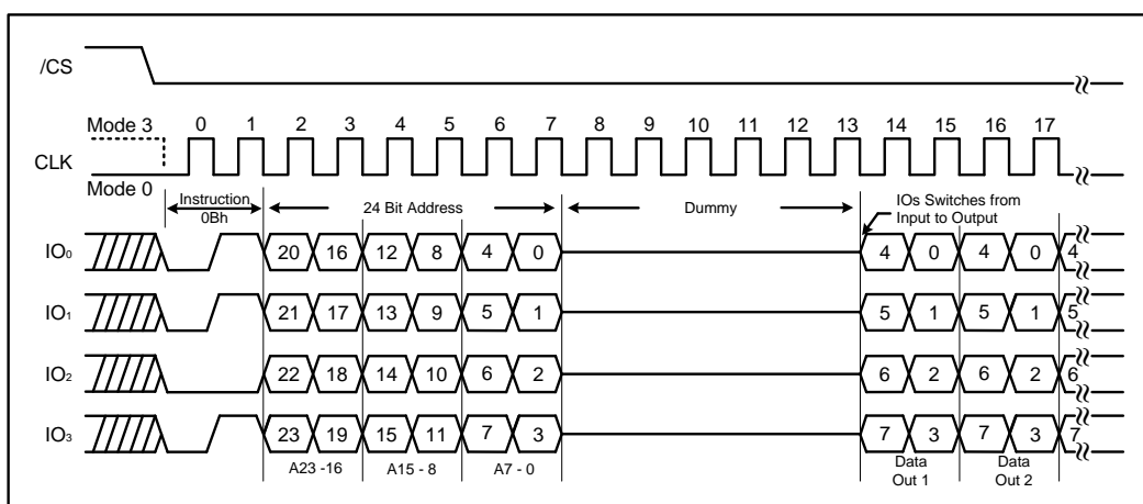
Figure 13c. Fast Read instruction (QPI Mode, 108MHz)
