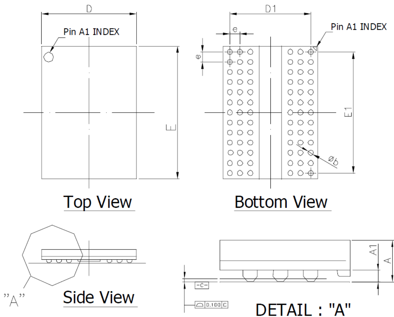
Figure 105. 78-Ball FBGA Package 7.5x10.5x1.0mm(max) Outline Drawing Information
