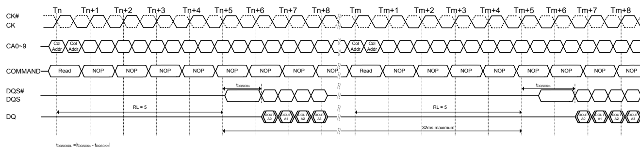
Figure 15. t_{DQSCKDL} timing
