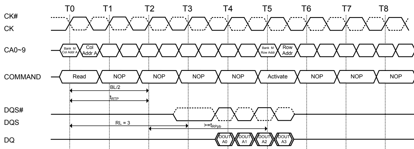
Figure 31. Burst read with auto-precharge (RL = 3, BL = 4, RU(t_{RTP}(\min)/t_{CK}) = 2 )
