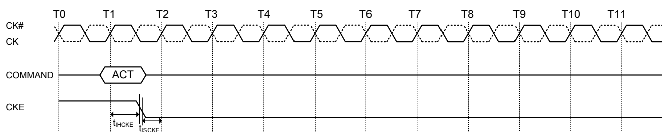
Figure 52. Activate command to power-down entry
