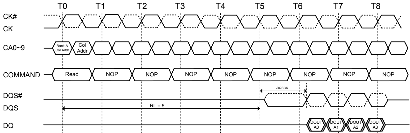
Figure 13. Burst read (RL = 5, BL = 4, t_{DQSCK} > t_{CK} )
