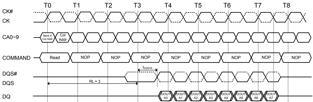
Figure 14. Burst read (RL = 3, BL = 8, t_{DQSCK} < t_{CK} )
