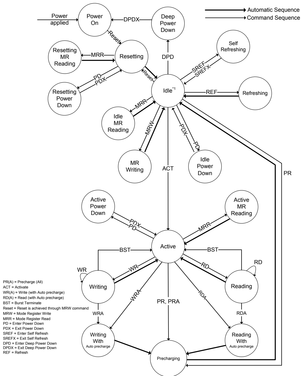
Figure 3. State Diagram
