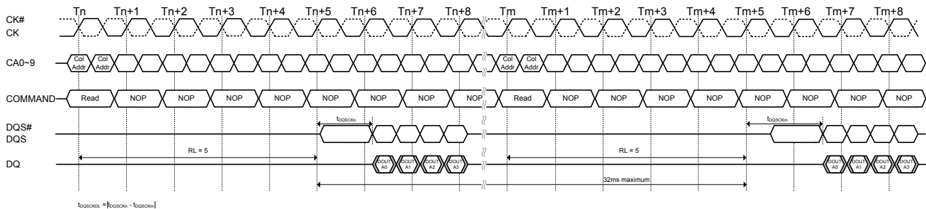
Figure 15. t_{DQSCKDL} timing
