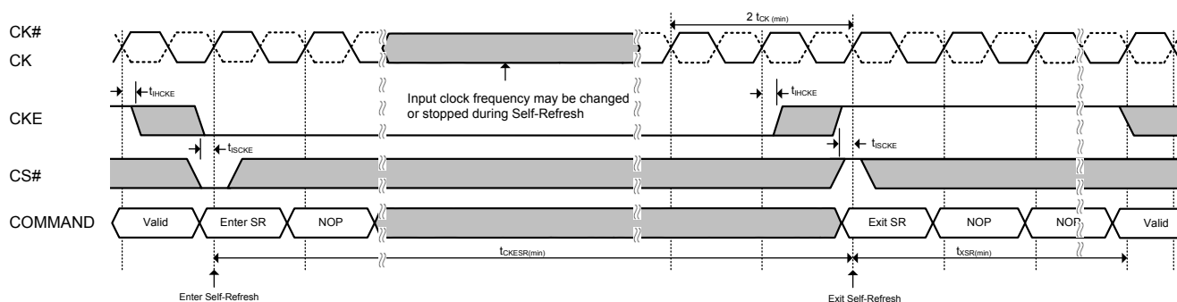
Figure 35. Self-Refresh Operation
