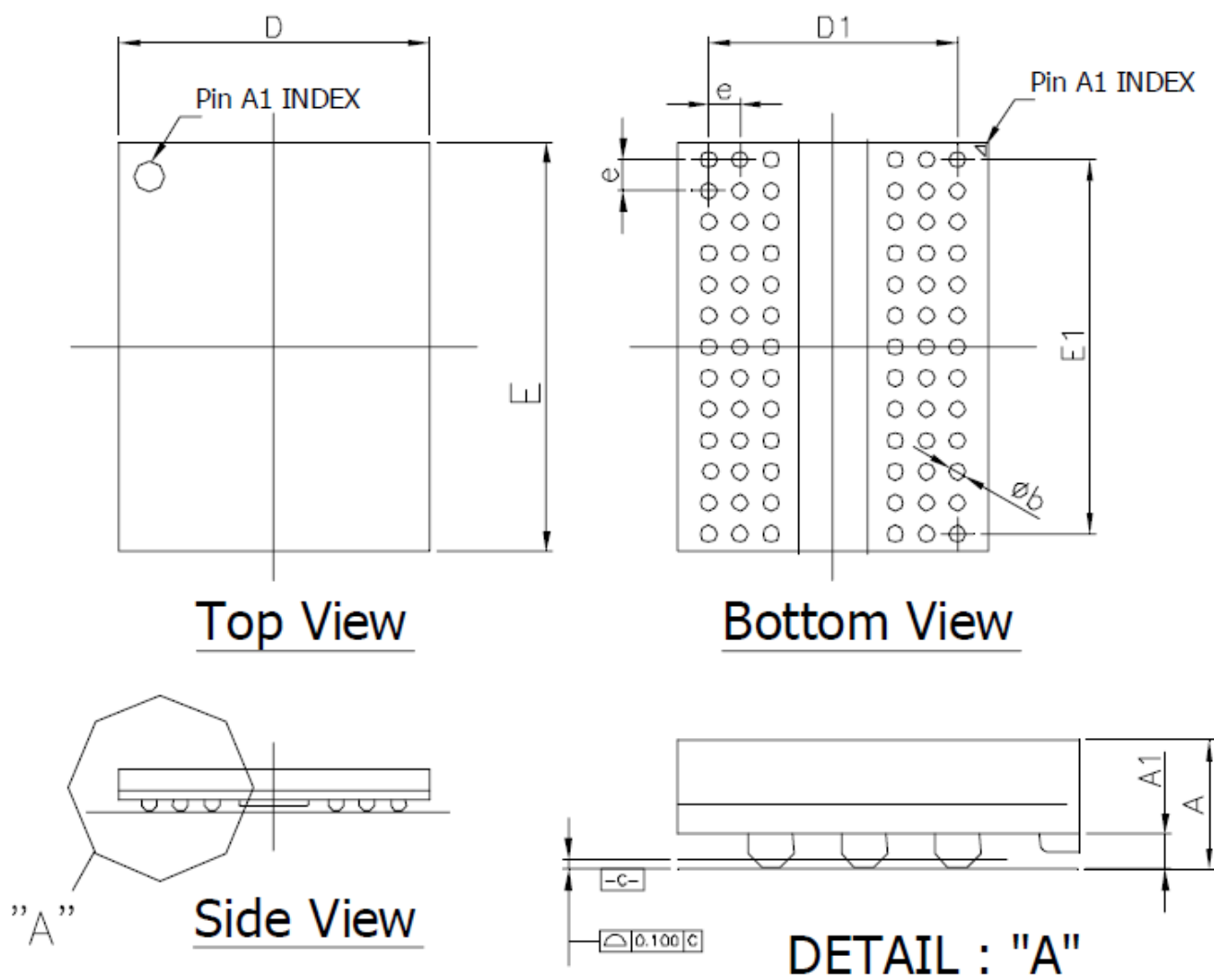
Figure 82. 78-Ball FBGA Package 8x10.5x1.0mm(max) Outline Drawing Information
