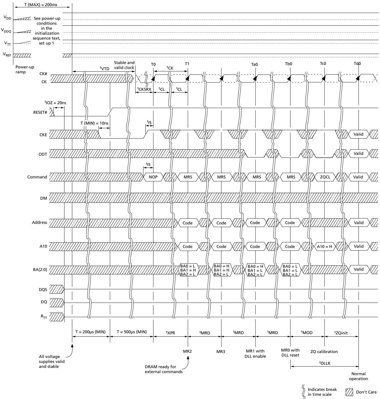
Figure 46: Initialization Sequence
