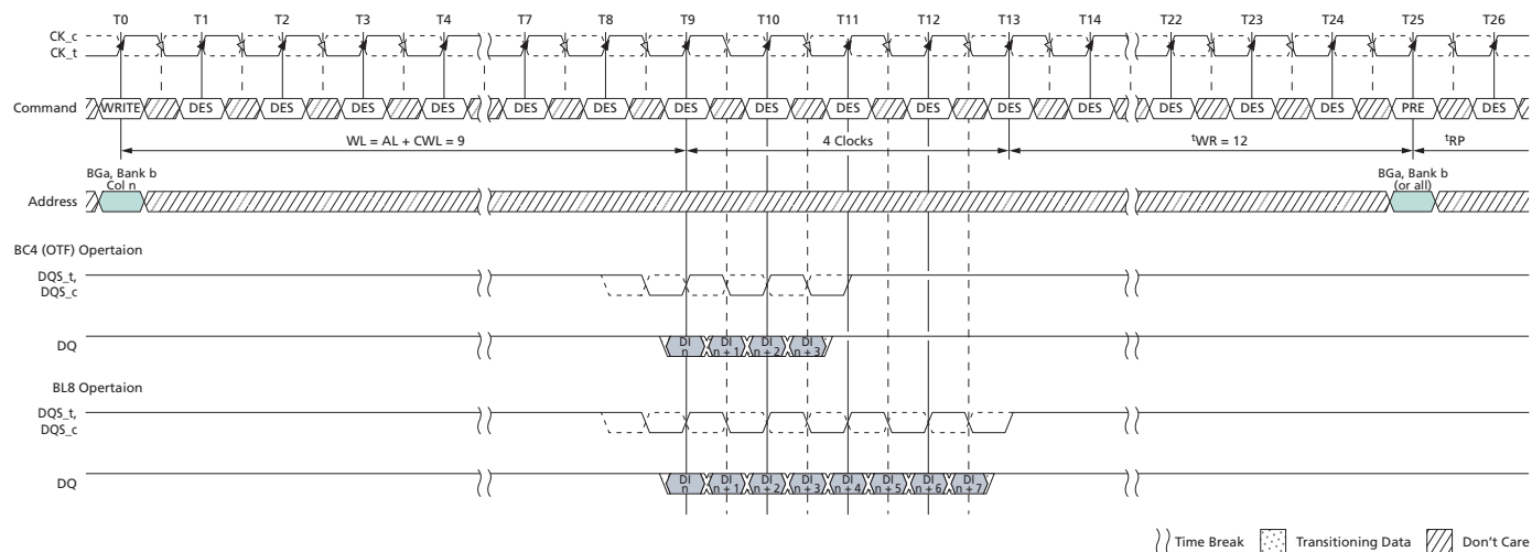
Figure 183: WRITE (BL8/BC4-OTF) to PRECHARGE with 1t_{CK} Preamble
