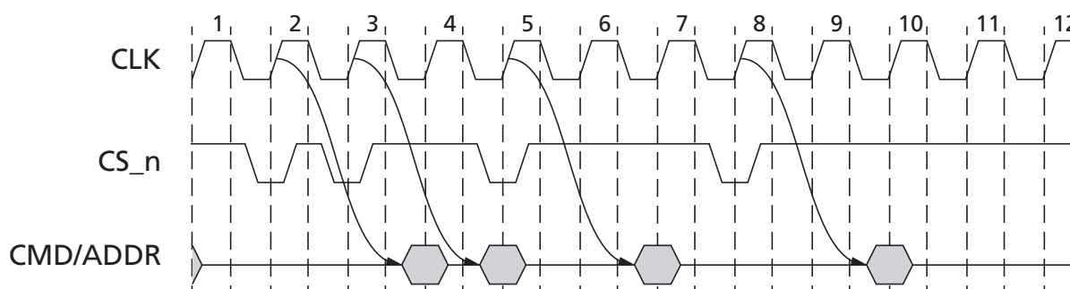
Figure 21: CAL Timing Example (Consecutive \text{CS}_n = LOW)
