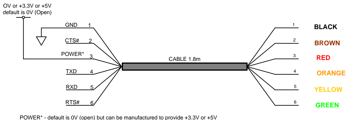
Figure 4.1 USBC-FS-RS232-0V-1800-WE Connections
