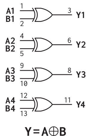
Figure 1: AP54RHC86 logic diagram
