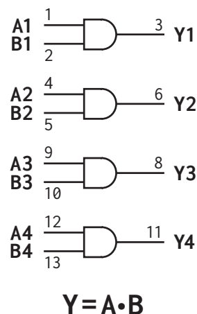
Figure 1: AP54RHC08 logic diagram
