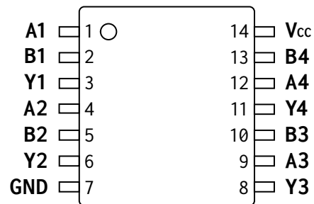
Figure 2: AP54RHC08 device pinout overview
