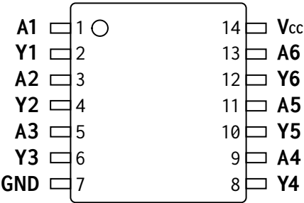
Figure 2: AP54RHC04 Device Pinout
