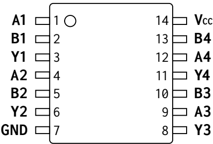
Figure 2: AP54RHC00 Device Pinout
