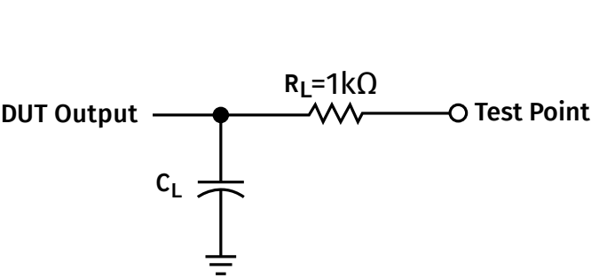
Figure 3: Load Circuit
