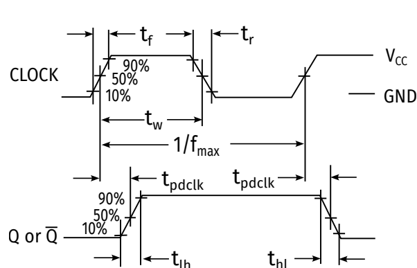
Figure 3: Timing measurements
