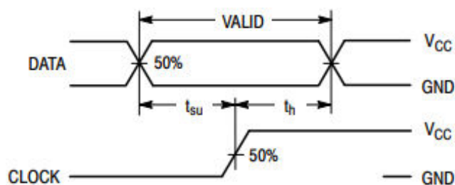
Figure 5: Setup and hold time measurement
