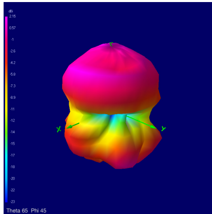
3700 MHz
