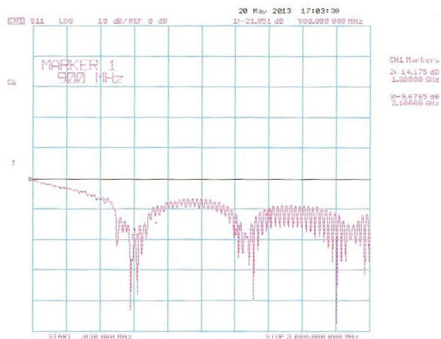
GSM Return Loss Graph
