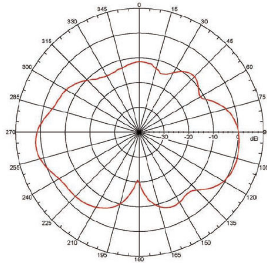
GSM Far-field amplitude at 1800 MHz
