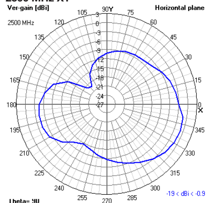
2500 MHz XY
