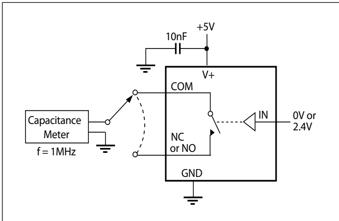
Figure 7. Channel-Off Capacitance
