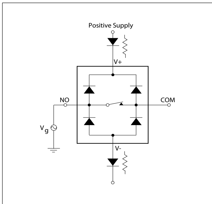
Figure 1. Overvoltage Protection
