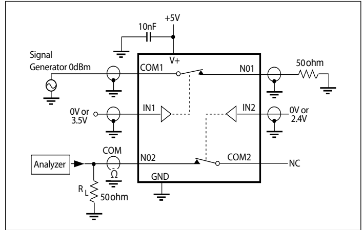
Figure 6. Crosstalk
