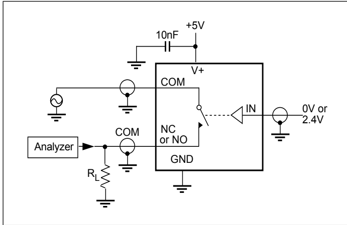
Figure 5. Off Isolation
