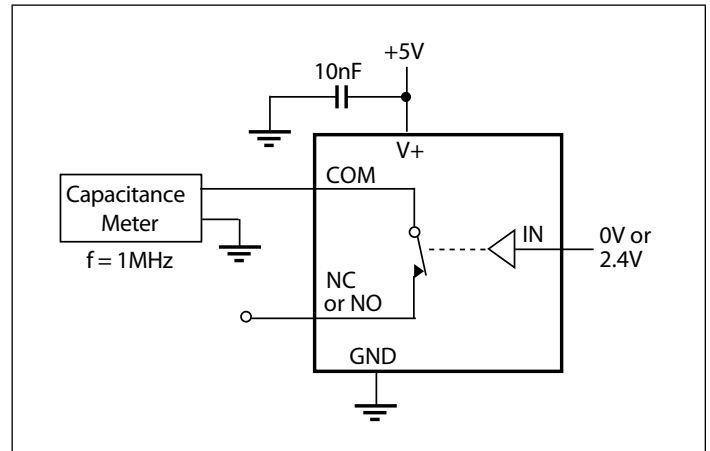
Figure 8. Channel-On Capacitance
