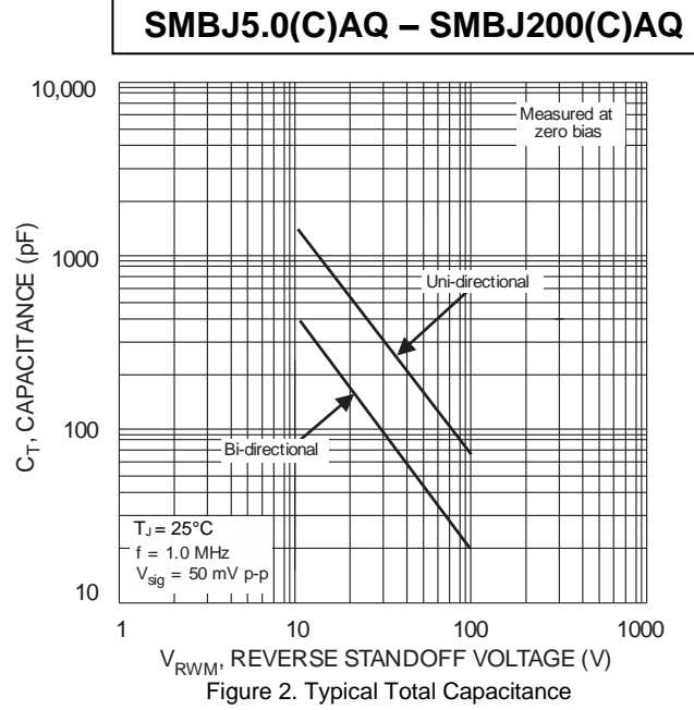
Figure 2. Typical Total Capacitance
