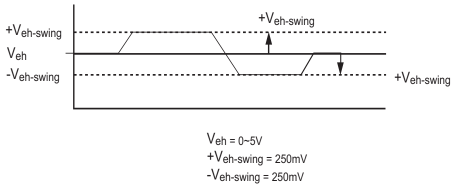
ARC single mode signal output waveform
