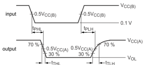
Figure 2: Propagation Delay and Transition Times B→A
