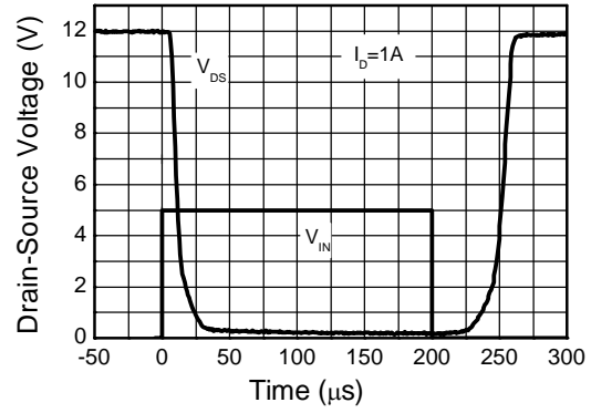
Switching Speed
