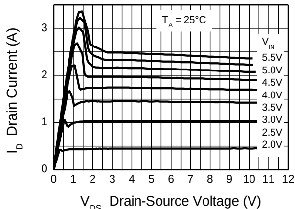
Typical Output Characteristic
