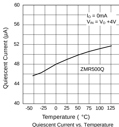
Quiescent Current vs. Temperature
