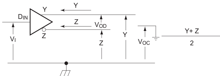
Figure 1. Driver Voltage and Current Definitions
